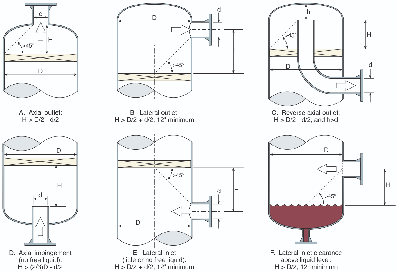
Figure 24. Generally accepted spacing guidelines to maintain even velocity profile and avoid entrainment in mist eliminators in cylindrical vessels with axial flow
