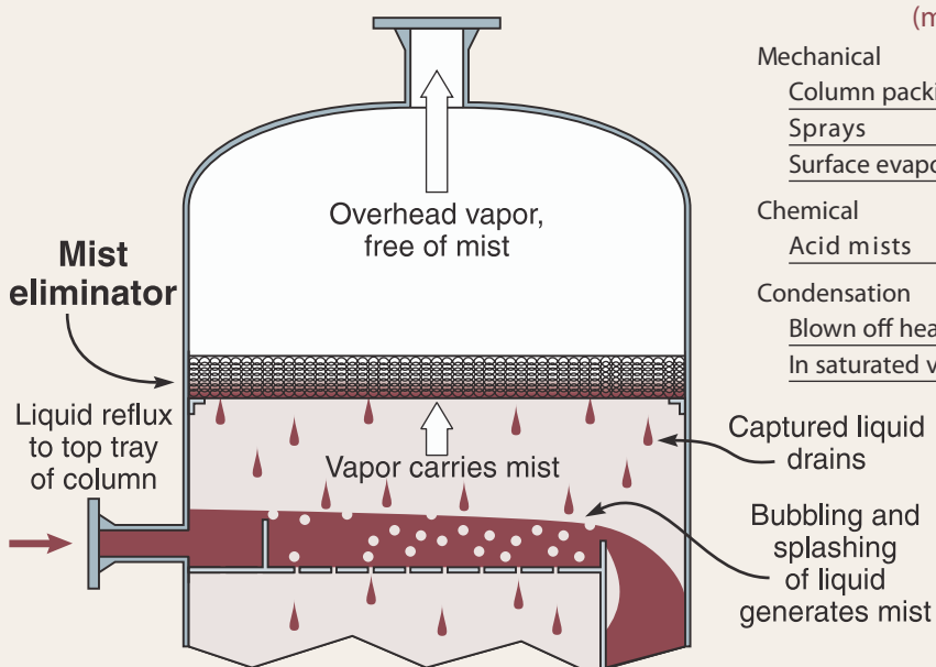
Figure 1. Typical mist eliminator application in distillation column
