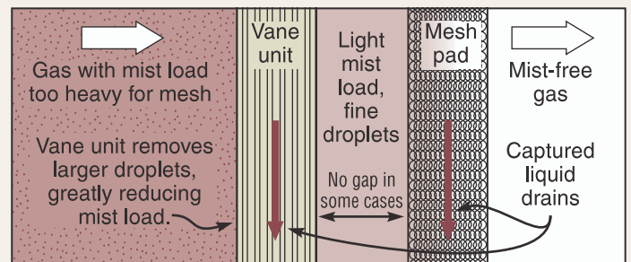
Figure 21. Shielding a mesh pad from a very heavy mist load with a vane unit ahead
