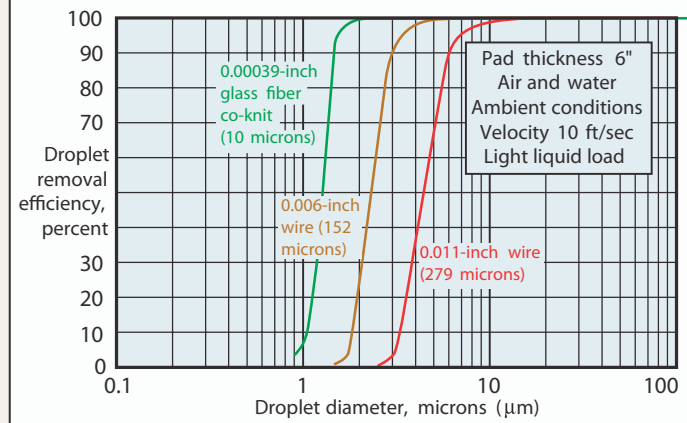
Figure 13. Examples of variation of droplet capture efficiency with droplet size and filament diameter
